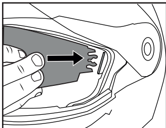
2_ INSTALL IN THE SLOT ON BOTH SIDES
